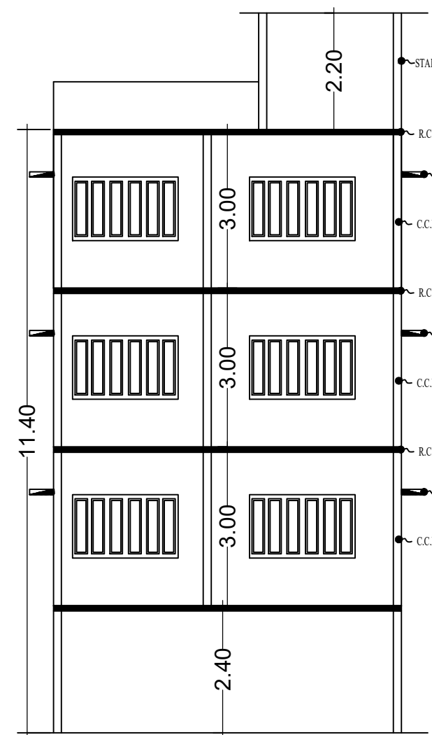
SECTION @ X-X'
